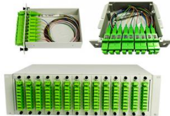
LGX box LGX box/ PLC patch panel, 19" rack PLC patch panel
