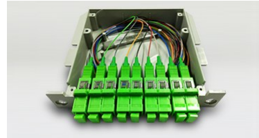
LGX PLC splitter with SC APC connector
