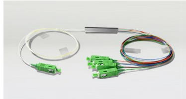
PLC splitter with SC APC connector
